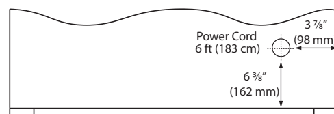
Cabinet Cut-Out
