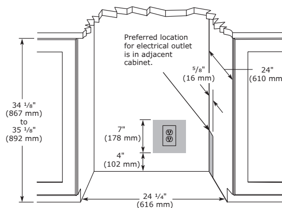
Cabinet Cut-Out
