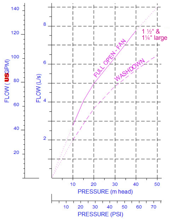
Performance Curve (large hose nozzle)
