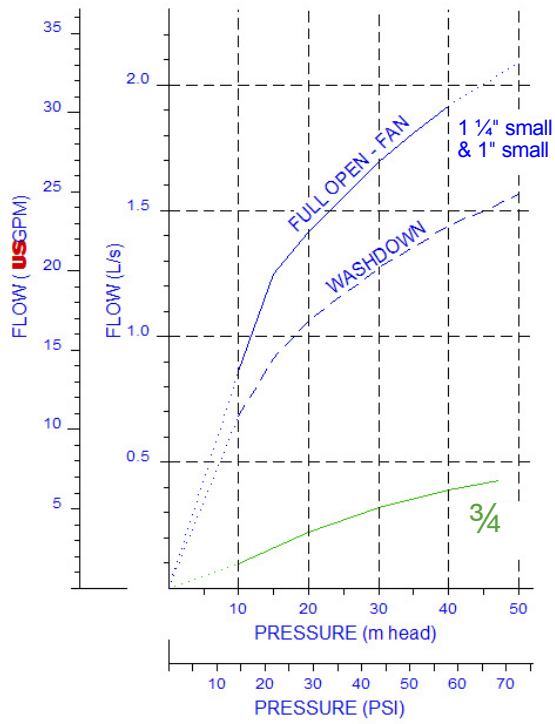
Performance Curve (small hose nozzle)
